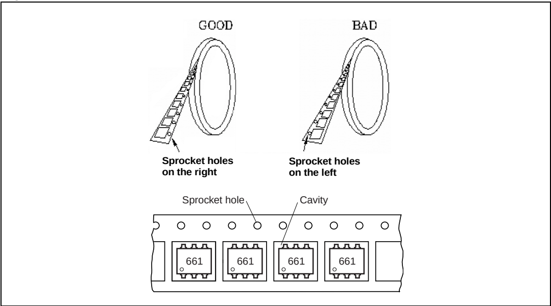
Figure 20. Device orientation
