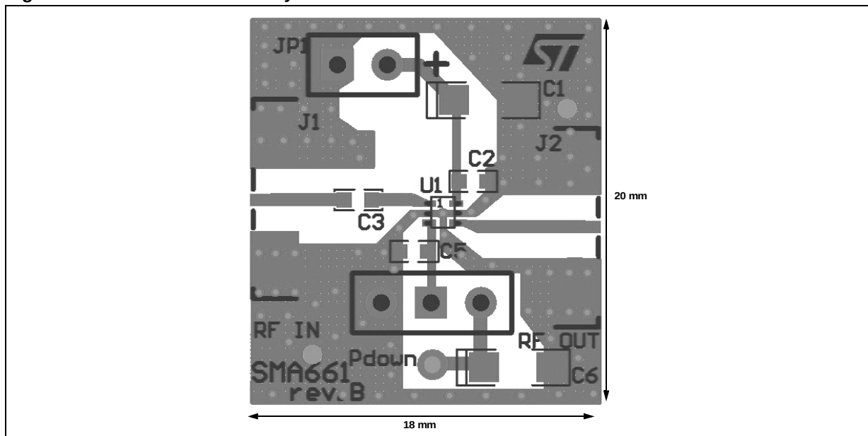
Figure 14. Evaluation Board Layout
